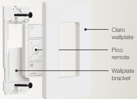
Pico remote wall-mounting kit (sold separately)
